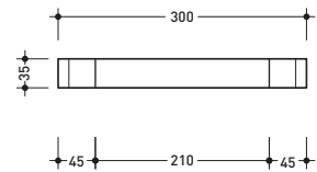
vista frontale / frontal view
