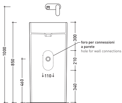
vista frontale / frontal view
