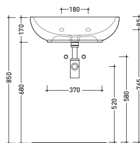
vista frontale / frontal view
