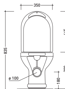
vista retro / back view
