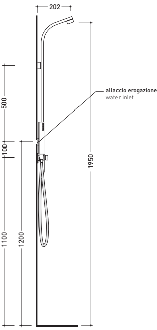
vista laterale / lateral view
