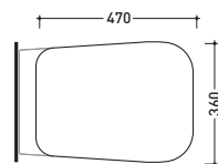
art. CM118 vista zenitale / zenital view
