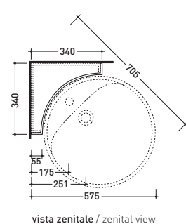
vista zenitale / zenital view
