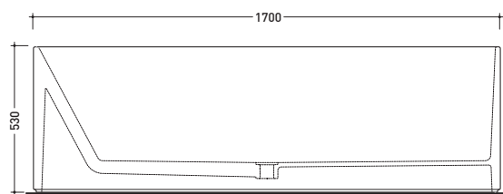
vista frontale / frontal view
