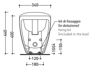
vista retro / back view
