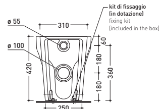
vista retro / back view
