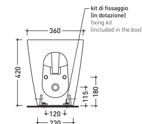
vista retro / back view
