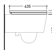
art. 5064 vista laterale / lateral view
