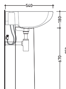
vista laterale / lateral view
