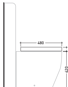
art. TR117 + TR39 vista laterale / lateral view
