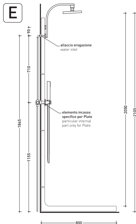
vista laterale / lateral view
