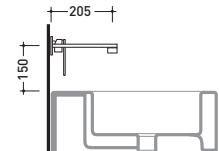
vista laterale / lateral view
