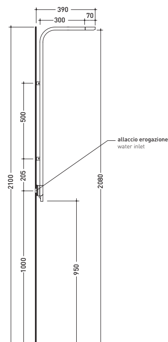
vista laterale / lateral view
