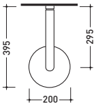
vista zenitale / zenital view
