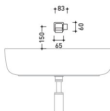
vista frontale / frontal view
