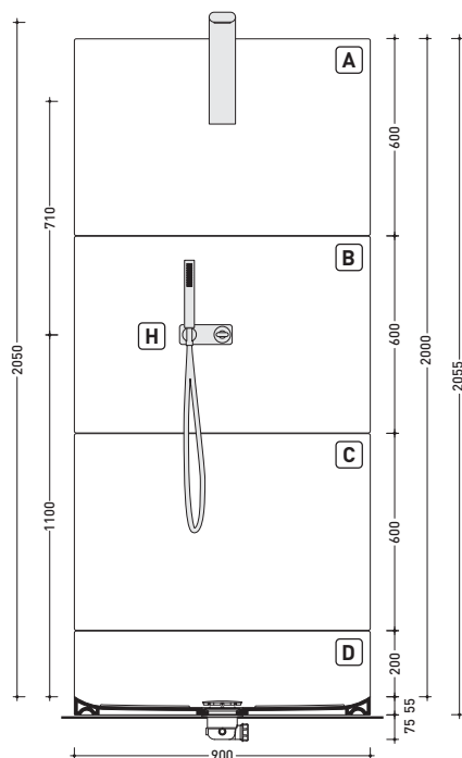
vista frontale / frontal view
