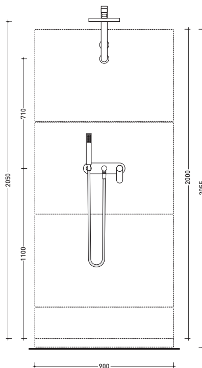
vista frontale / frontal view
