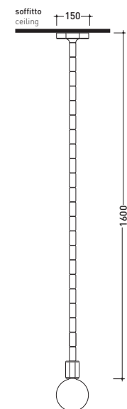
vista frontale / frontal view
