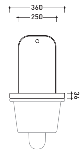
vista frontale / frontal view
