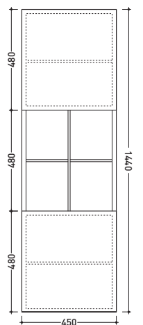
vista frontale / frontal view
