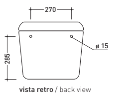
vista retro / back view
