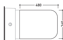
art. TR117 + TR39 vista zenitale / zenital view
