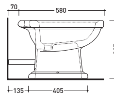
vista laterale / lateral view
