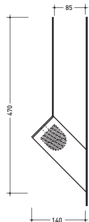
vista laterale / lateral view
