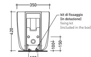
vista retro / back view
