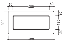
vista frontale / frontal view
