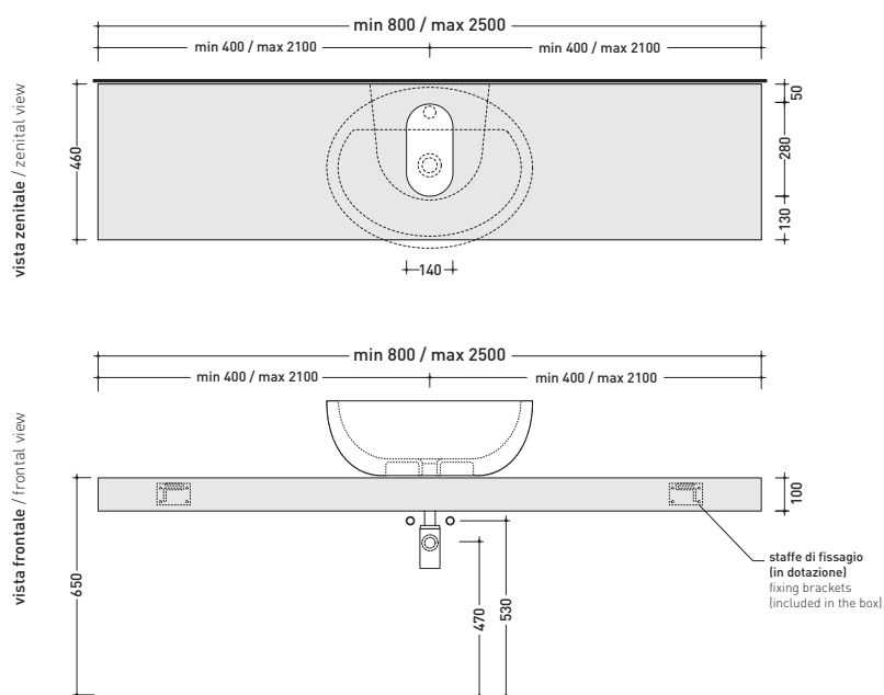
FORTY6 mensola da cm 80 a 250 art. F6DP per lavabi Dip (DP481/DP482) shelf from 80 to 250 cm to suit Dip basins (DP481/DP482)
