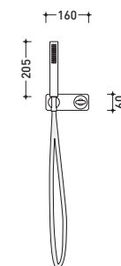
vista frontale / frontal view
