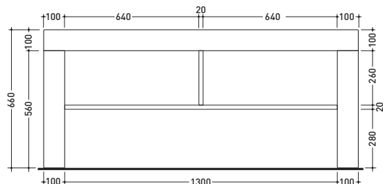
vista frontale / frontal view
