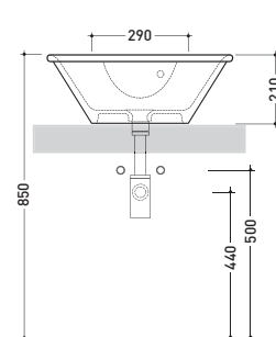
vista frontale appoggio frontal view bench version
