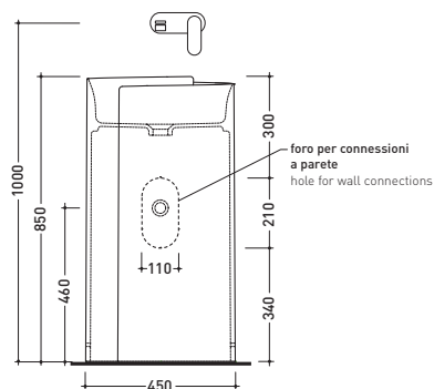
vista frontale / frontal view
