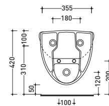
vista retro / back view
