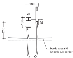
vista frontale / frontal view
