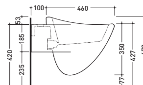
vista laterale / lateral view
