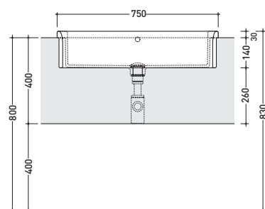
vista frontale / frontal view
