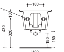
vista retro / back view
