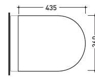
art. 5064 vista zenitale / zenital view
