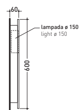
vista laterale / lateral view
