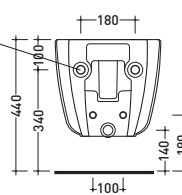
vista retro / back view
