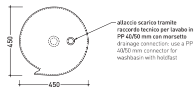
vista zenitale / zenital view
