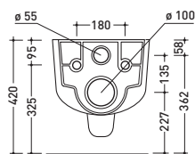
vista retro / back view
