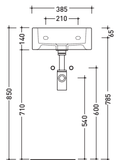
vista frontale / frontal view
