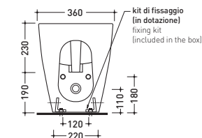
vista retro / back view
