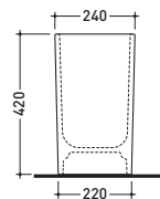
vista frontale / frontal view
