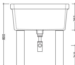
vista frontale / frontal view
