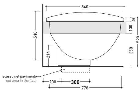
vista laterale / lateral view
