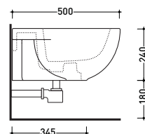
vista laterale / lateral view
