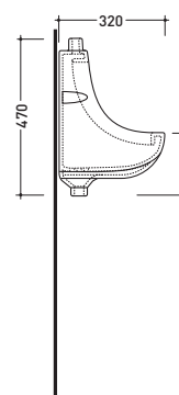
vista laterale / lateral view
