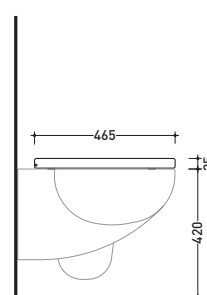
art. SR118 vista laterale / lateral view
