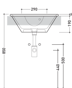
vista frontale incasso frontal view vanity version
