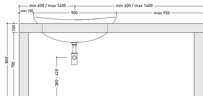
vista frontale / frontal view
