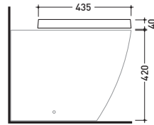
art. LK117 vista laterale / lateral view
