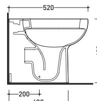
vista laterale / lateral view
