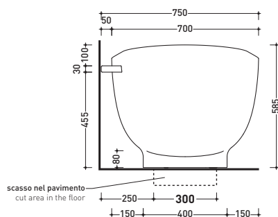
vista laterale / lateral view
