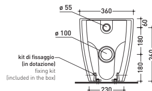
vista retro / back view
