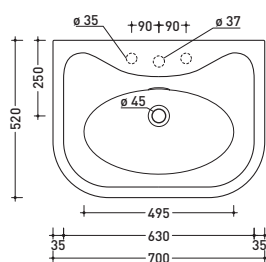
vista zenitale / zenital view
