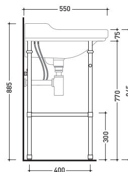
vista laterale / lateral view
