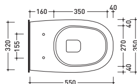
vista zenitale / zenital view
