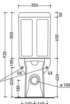
vista retro / back view
