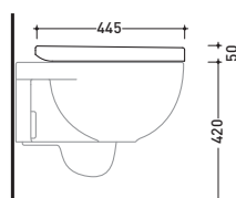
vista laterale / lateral view
