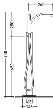
vista laterale / lateral view
