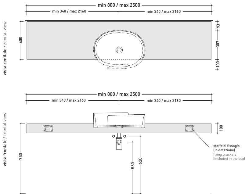
FORTY6 mensola da cm 80 a 250 x 40 art. F6RL56S per lavabo Roll 56 semincasso (RL56S) shelf from 80 to 250 x 40 cm to suit Roll 56 semi-inset basin (RL56S)
