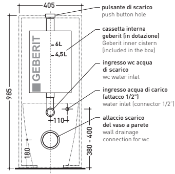
vista frontale parete / wall frontal view
