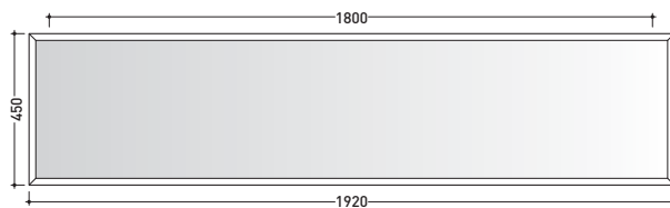
vista frontale / frontal view
