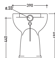
vista retro / back view
