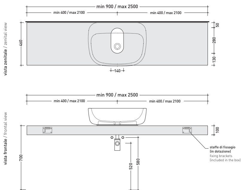
FORTY6 mensola da cm 90 a 250 art. F6MN64 per lavabo Mono' 64 (MN64L) shelf from 90 to 250 cm to suit Mono' 64 basin (MN64L)
