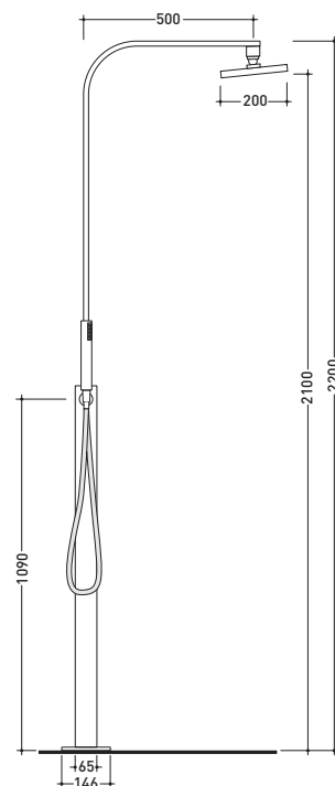
vista laterale / lateral view
