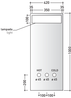
vista frontale / frontal view
