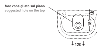
vista zenitale / zenital view
