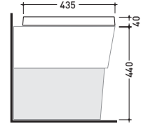
art. 5064A vista laterale / lateral view
