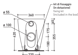
vista retro / back view
