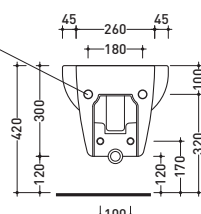
vista retro / back view
