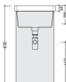
vista frontale / frontal view
