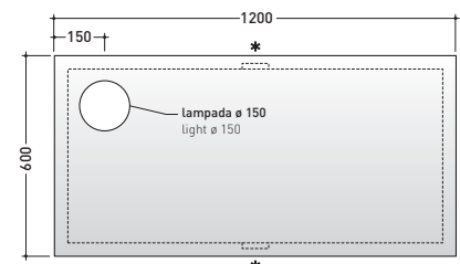
vista frontale / frontal view
