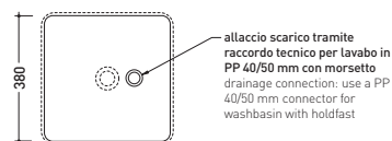
vista zenitale / zenital view
