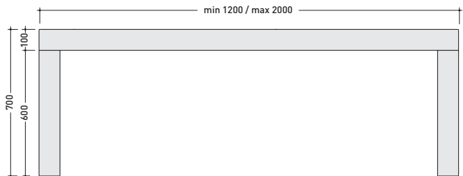
vista frontale / frontal view
