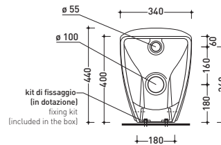
vista retro / back view
