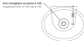
vista zenitale / zenital view
