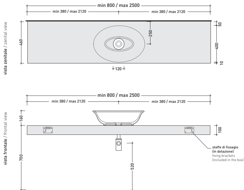
FORTY6 mensola da cm 80 a 250 art. F6BL per lavabi Boll (BL42L/BL44L/BL56L) shelf from 80 to 250 cm to suit Boll basins (BL42L/BL44L/BL56L)
