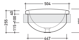
vista laterale / lateral view
