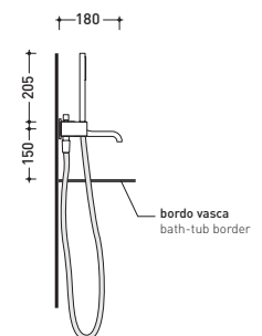
vista laterale / lateral view
