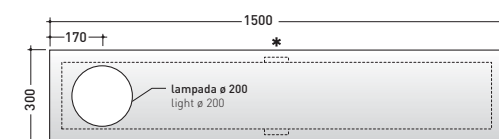
vista frontale / frontal view
