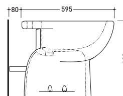
vista laterale / lateral view
