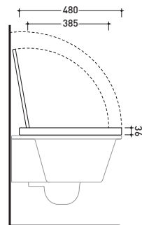
vista laterale / lateral view
