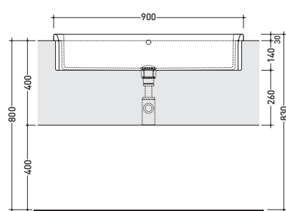
vista frontale / frontal view
