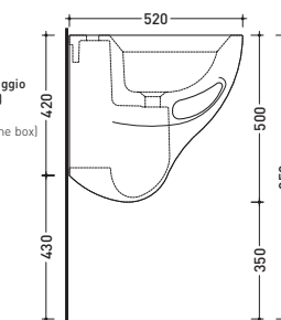
vista laterale / lateral view
