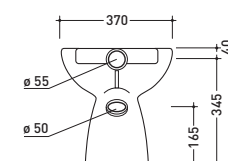
vista retro / back view
