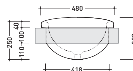
vista laterale / lateral view
