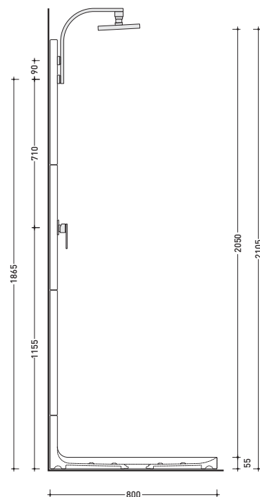
vista laterale / lateral view
