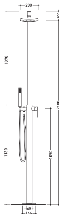
vista frontale / frontal view
