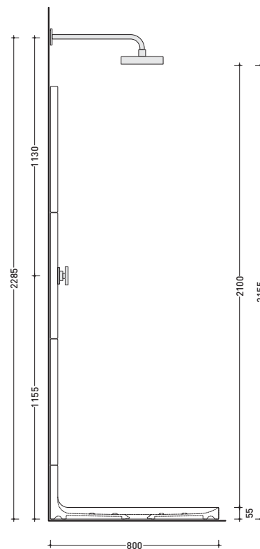
vista laterale / lateral view
