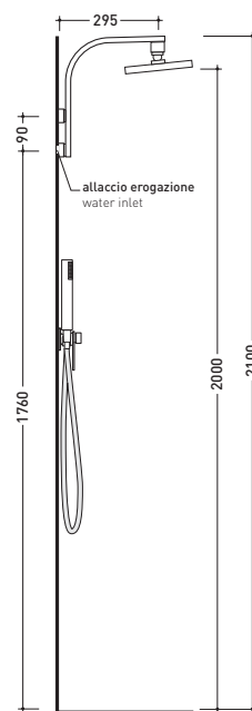
vista laterale / lateral view
