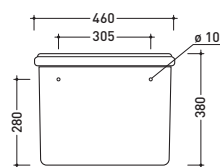
vista retro / back view
