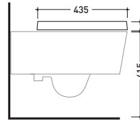
art. 5051/WC vista laterale / lateral view
