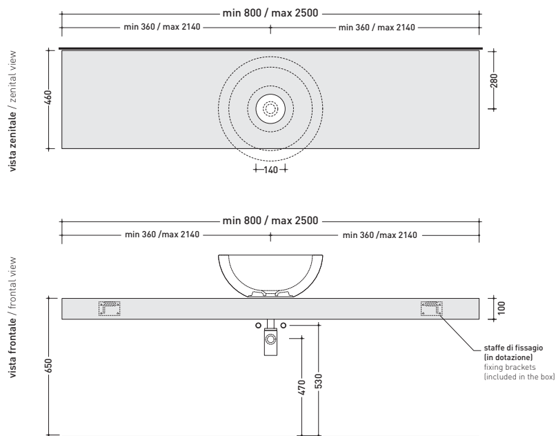
FORTY6 mensola da cm 80 a 250 art. F6FNT per lavabi Fonte (FN50L/FT52L) shelf from 80 to 250 cm to suit Fonte basins (FN50L/FT52L)
