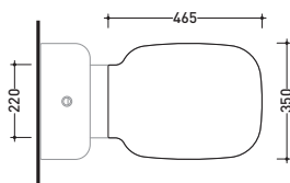
art. SR115 / SR116 vista zenitale / zenital view
