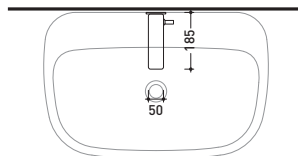
vista zenitale / zenital view
