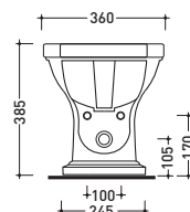
vista retro / back view
