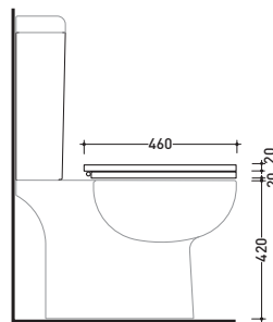
art. SR115 / SR116 vista laterale / lateral view
