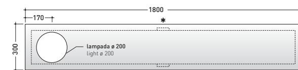
vista frontale / frontal view
