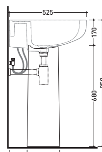
vista laterale / lateral view
