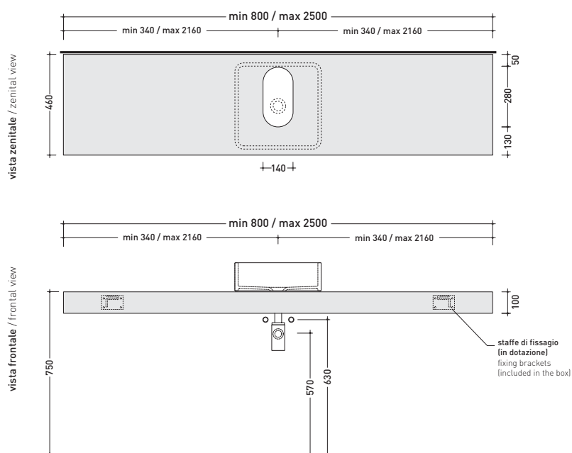
FORTY6 mensola da cm 80 a 250 art. F6MW per lavabi Miniwash (MWL40/MWL48) shelf from 80 to 250 cm to suit Miniwash basins (MWL40/MWL48)
