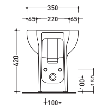
vista retro / back view
