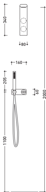
vista frontale / frontal view
