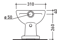
vista retro / back view
