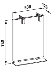
4195.1 2 Beleuchtungselemente Glas/Metall verchromt 2 lighting elements, glass with chrome-plated metal 2 éclairages verre/métal chromé 2 lampade in vetro/metallo cromato
